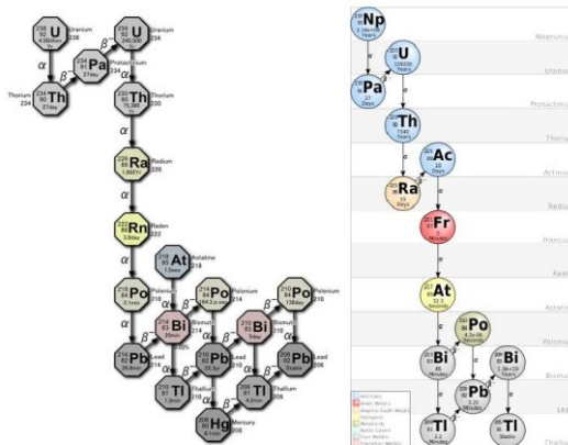
Figure 4-Uranium Decay Chain (left) and Neptunium Decay Chain (right)
